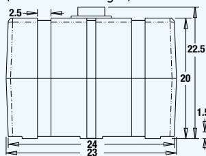
LS9 (Frame Mount 30 gal.)
